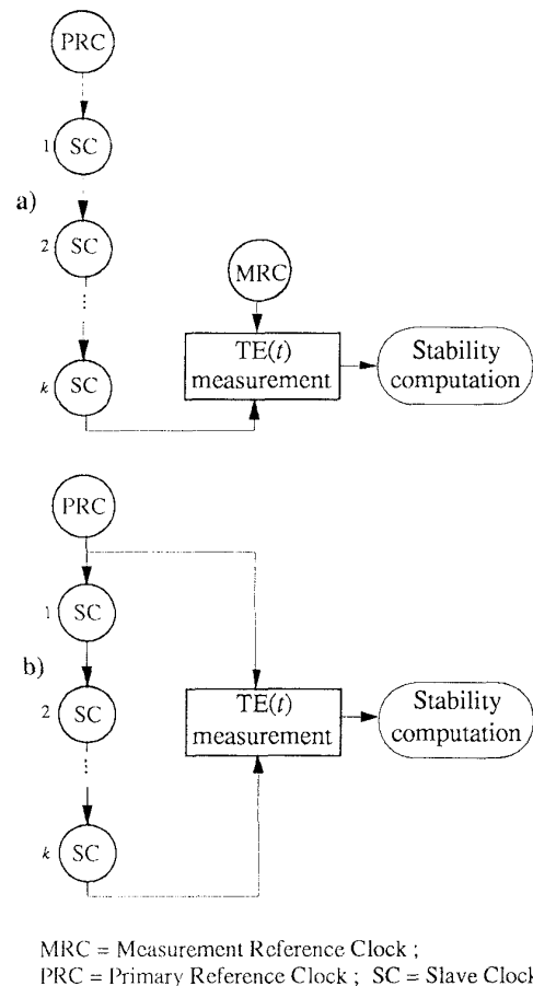
Fig.2 - Different configurations for synchronization network stability measurements.
