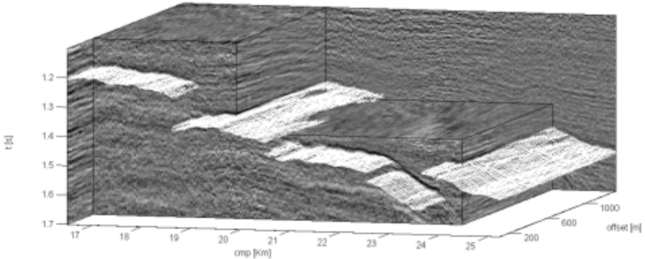
Figure 1 – HP for 2-D seismic surveys: picking of a multifaulted horizon on a 3-D prestack data volume.
