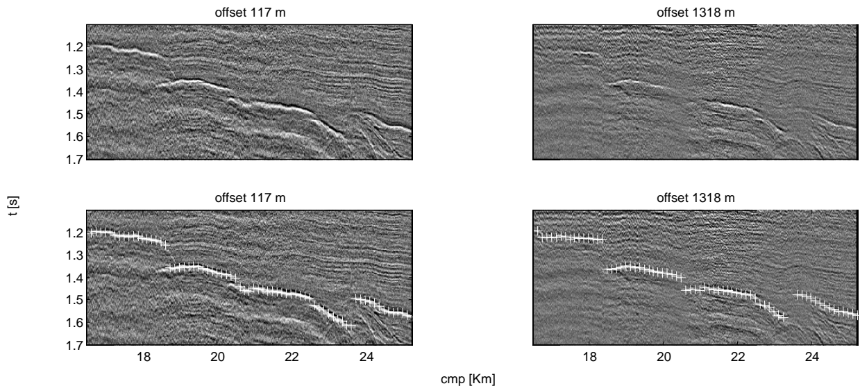
Figure 2 – Detailed view (offset slices) of 3-D data volume in fig.1: data (upper part) and estimated horizons (lower part).
