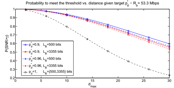
Fig. 3. Probability to meet a target beacon detection probability.
