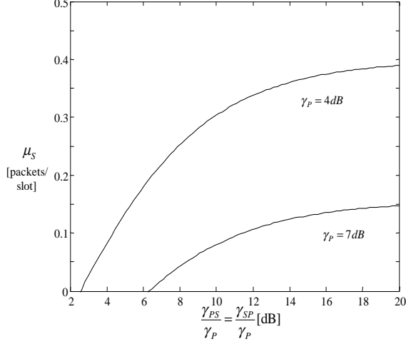
Fig. 4. Maximum throughput of the secondary user \mu_S for a fixed \lambda_P = \mu_P^{\max} versus the average channel gain ratios \gamma_{PS}/\gamma_P = \gamma_{SP}/\gamma_P ( \gamma_S = 10dB and \alpha = 0dB , \beta_P = \beta_S = 4dB ).
