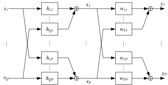
Fig. 1. Linear MIMO model for BSS
