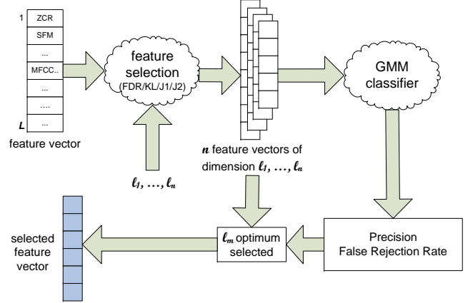
Figure 1: Hybrid feature selection system.
