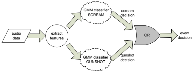
Figure 3: Classification scheme.
